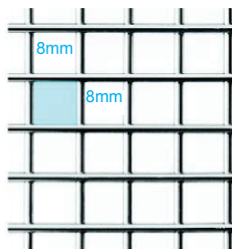
MESH SIZE 10MM X 10MM (ACTUAL SIZE) 8MM SPACE BETWEEN WIRES
